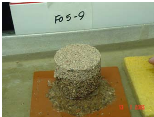
Figure 45B-4 Vaughan and Soares test on sample with good self-healing characteristics. As sample is submersed, capillary stresses are reduced and sample collapses quickly.
