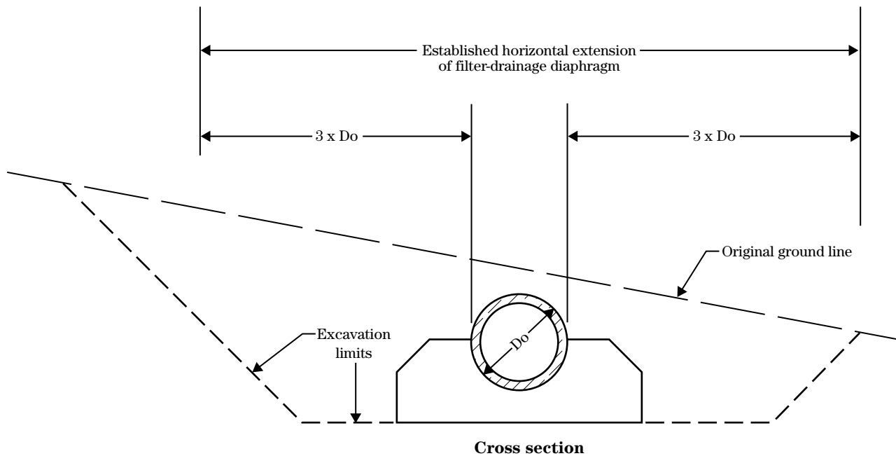
Figure 45A-1 Requirements for the horizontal extent of the filter diaphragm for rigid circular conduits
